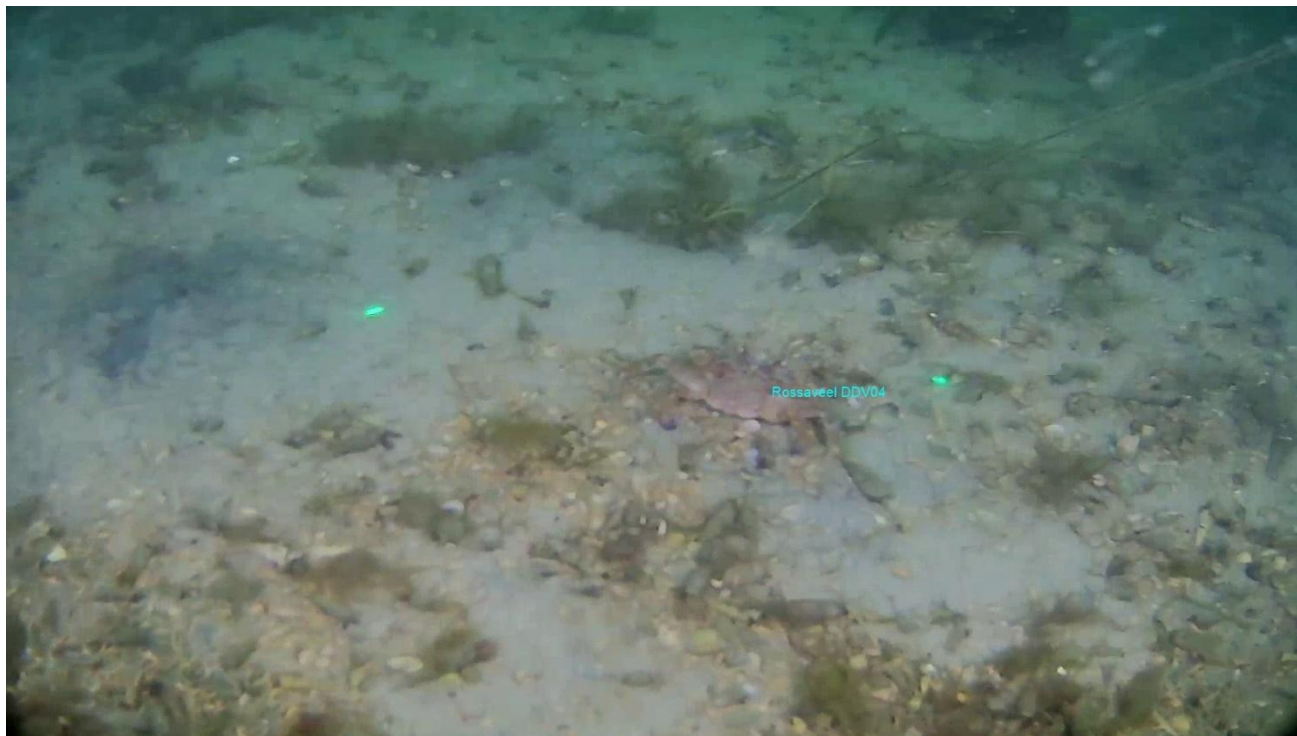
Figure 3.14: DDV Track 4 - sand substrate with shell debris, drift green macroalgae and solitary crab.
