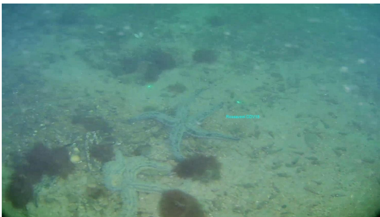
Figure 3.68: DDV Track 18 - mixed sediment substrate with filamentous red algae, auger shells ( Turitellinella tricarinata ), and Spiny starfish.
